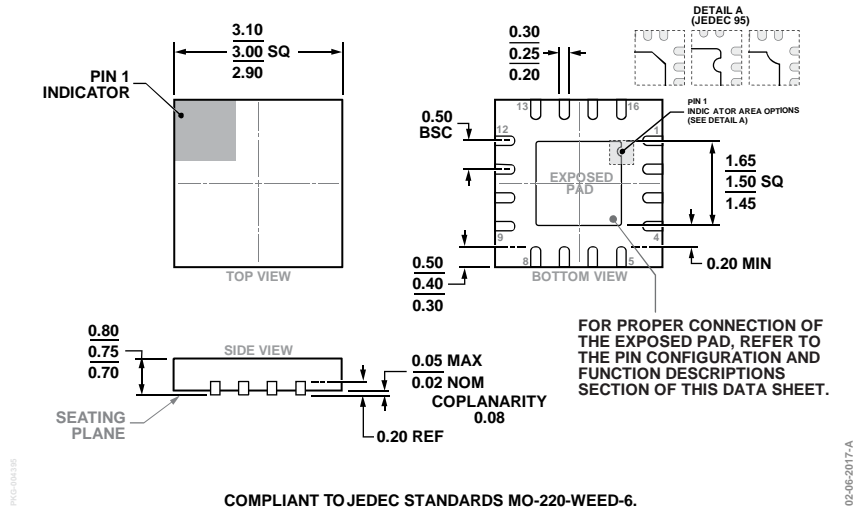
COMPLIANT TO JEDEC STANDARDS MO-220-WEED-6. Figure 48. 16-Lead Lead Frame Chip Scale Package [LFCSP] 3 mm x 3 mm Body and 0.75 mm Package Height (CP-16-27) Dimensions shown in millimeters
