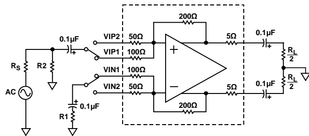
Figure 35. Single-Ended Input Loading Circuit
