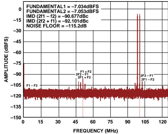
Figure 38. Measured Two-Tone Performance of the Circuit in Figure 40 for a 100 MHz and 102 MHz Input Signals
