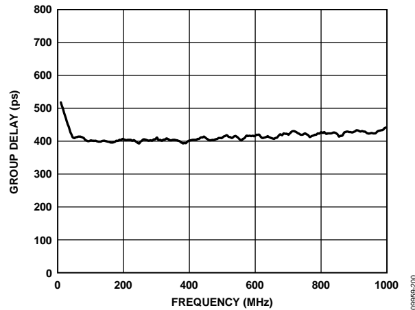
Figure 25. Group Delay vs. Frequency
