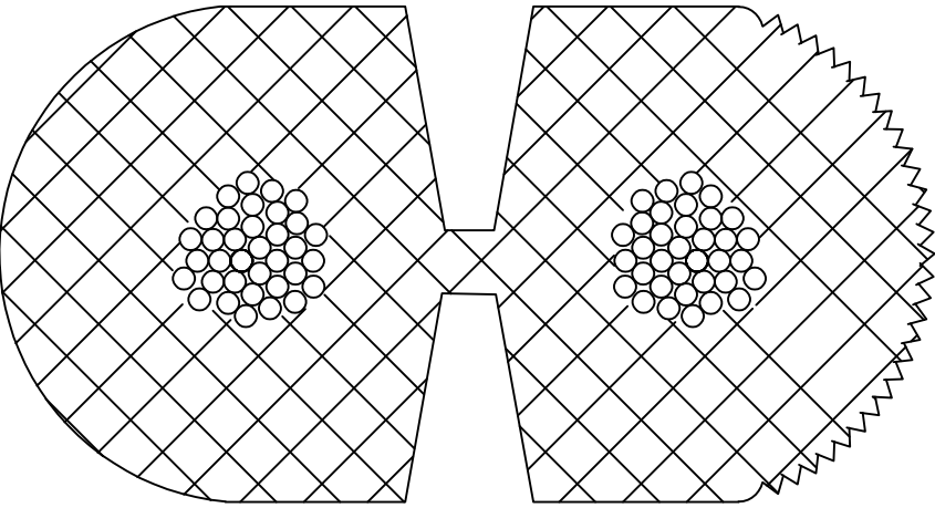
CROSS SECTION OF SPT-2 CABLE
