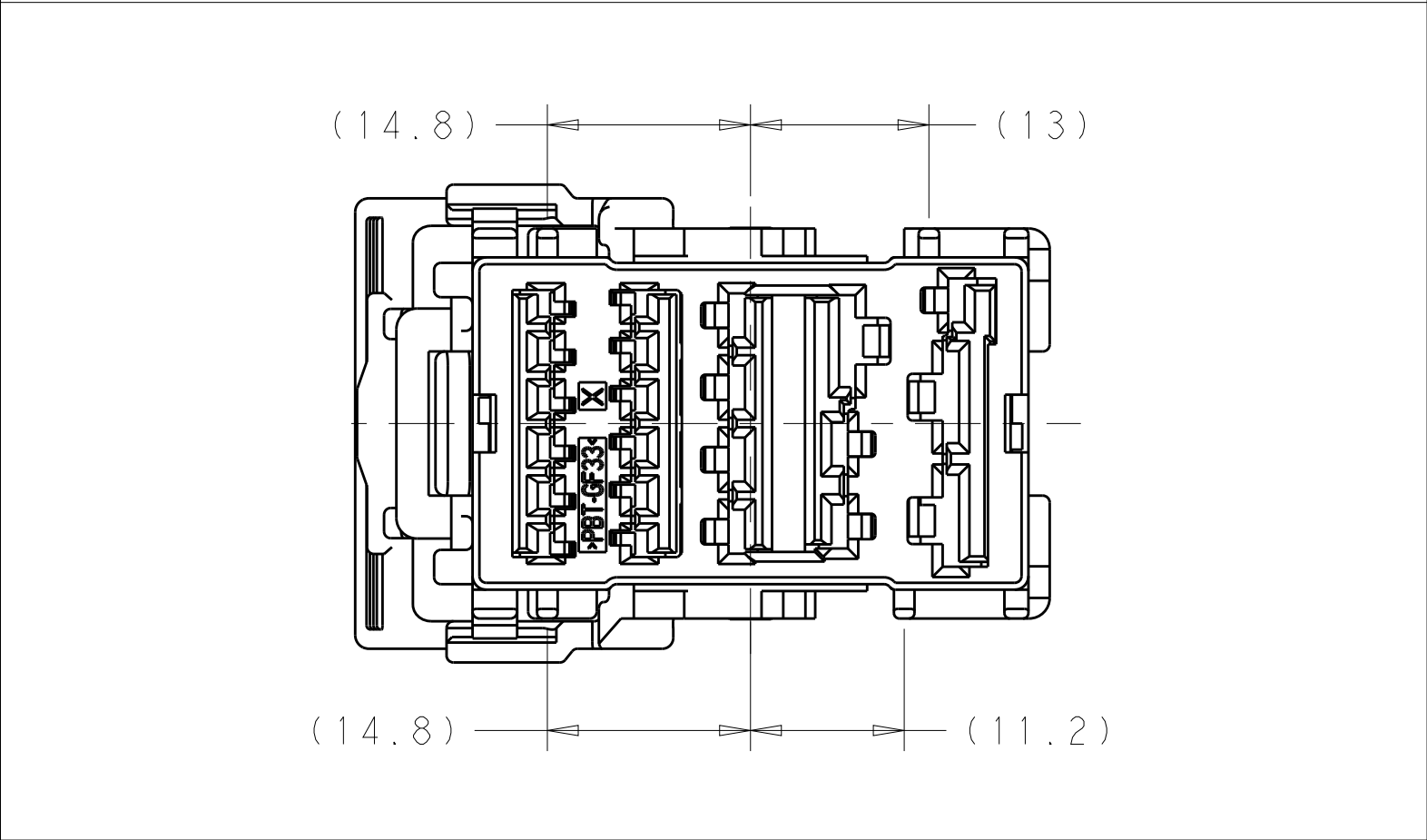
2098627-2 KEYING OPTION "B"
