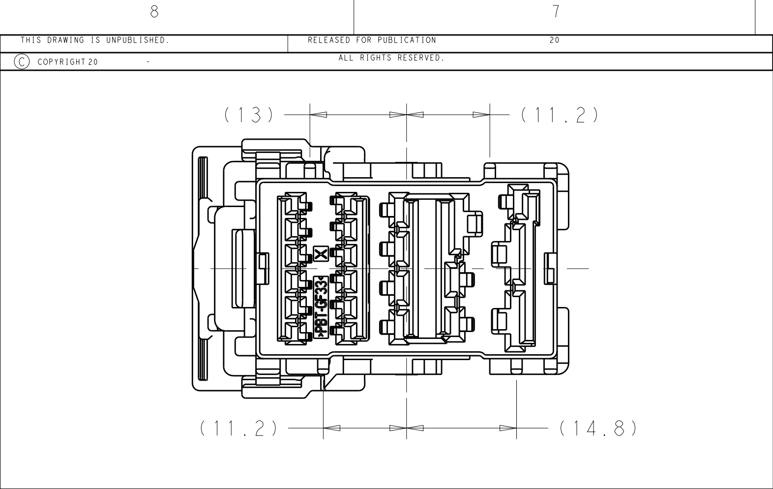
2098627-1 KEYING OPTION "A"
