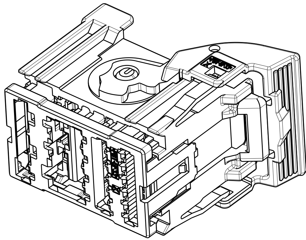
ISOMETRIC VIEWS
