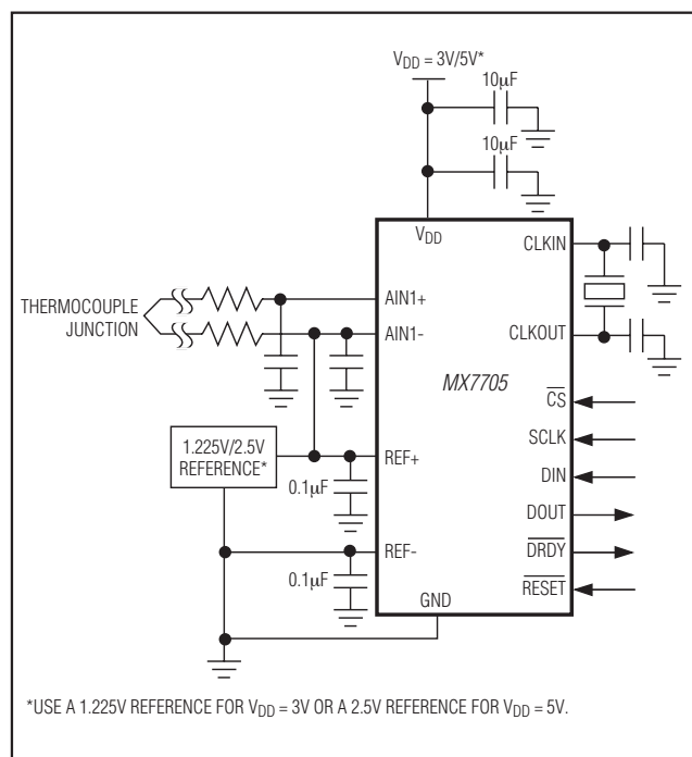
Figure 13. Temperature Measurement
