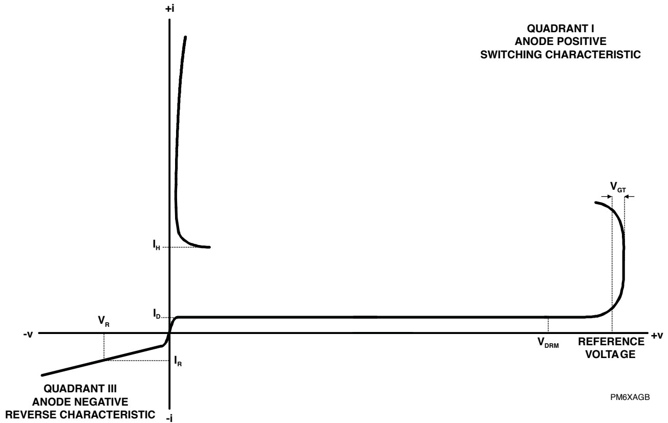
Figure 1. Voltage-Current Characteristic
