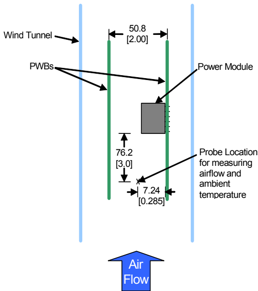
Figure 53. Thermal Test Set-up.
