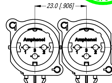
MIN MOUNTING PITCH (1:1)
