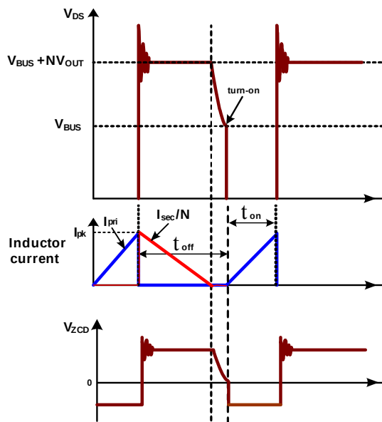
Figure 3: Boundary-Conduction Mode
