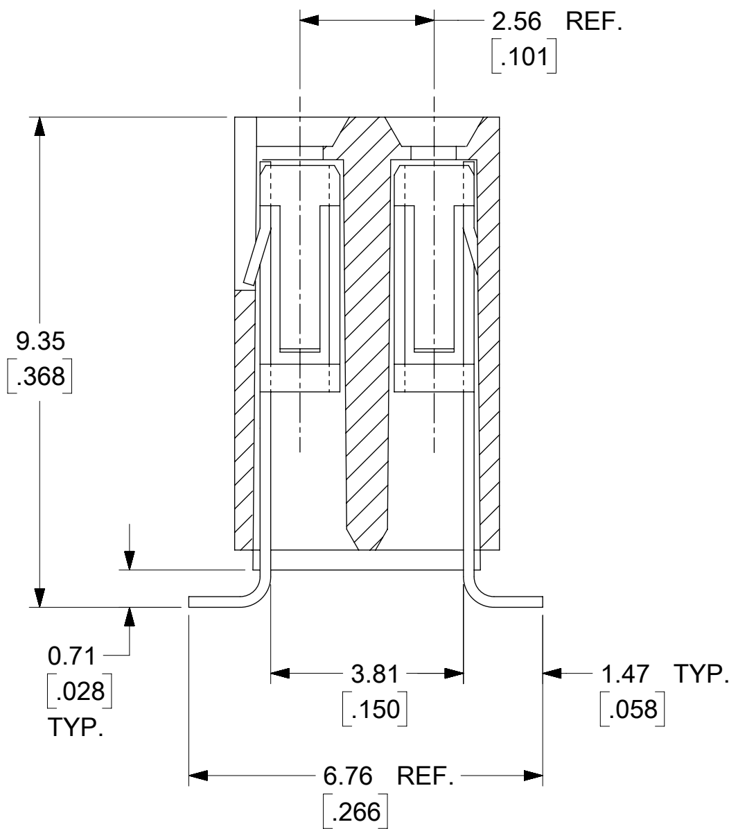
SECTION B-B
