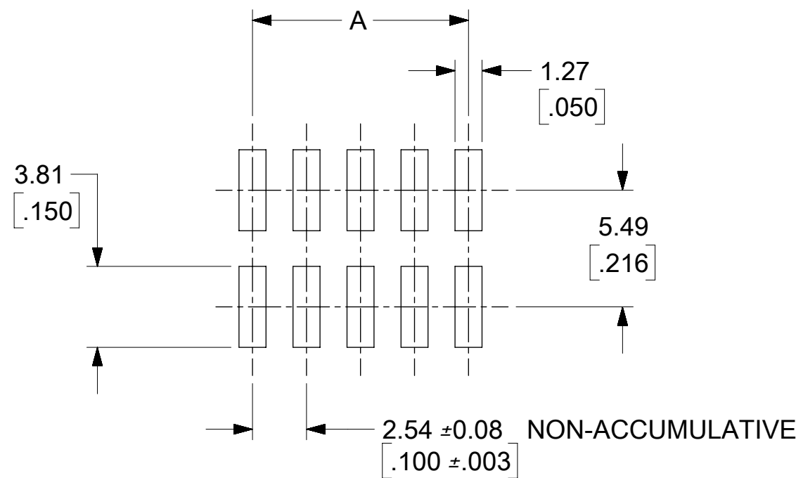
RECOMMENDED P.C. BOARD LAYOUT SCALE 4:1
