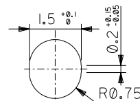
A部詳細 DETAIL A
