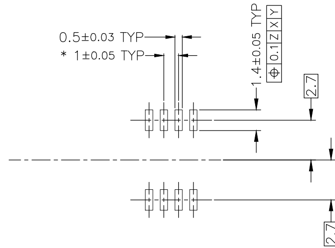
REFERENTIAL METAL MASK PAD OPENING (4:1)
