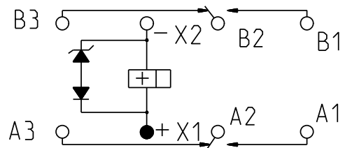
TERMINAL VIEW
