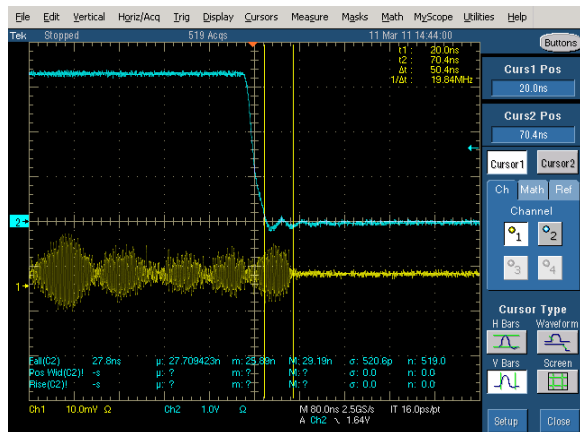
Figure 19. Power-Down Time
