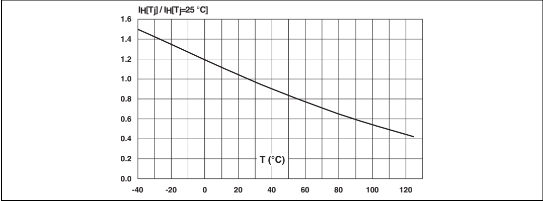
Figure 4. Relative variation of holding current versus junction temperature
