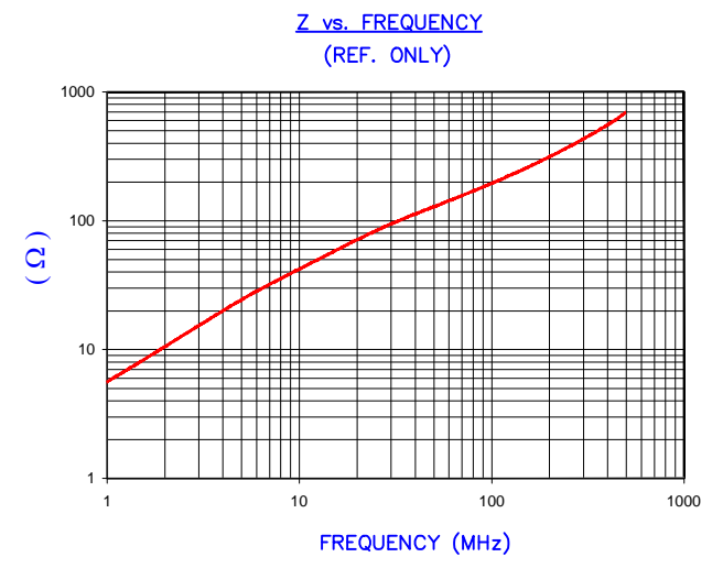
AGILENT E4991A Impedance/Material Analyzer HP 16092A Test Fixture, REF # 3013
