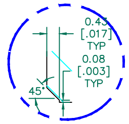
DETAIL "A" CHAMFER SCALE=6:1
