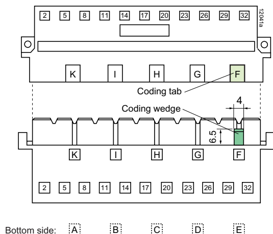
Fig. 18 Integrated code key system (H11 connector)
