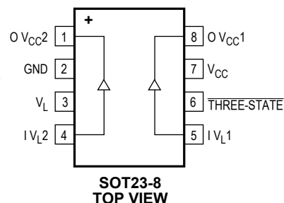
SOT23-8 TOP VIEW
