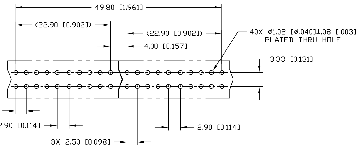
6 RECOMMENDED P.C. BOARD LAYOUT
