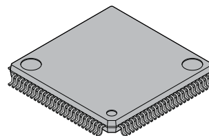
Plastic · LQFP, 100-pins (FPT-100P-M23)
