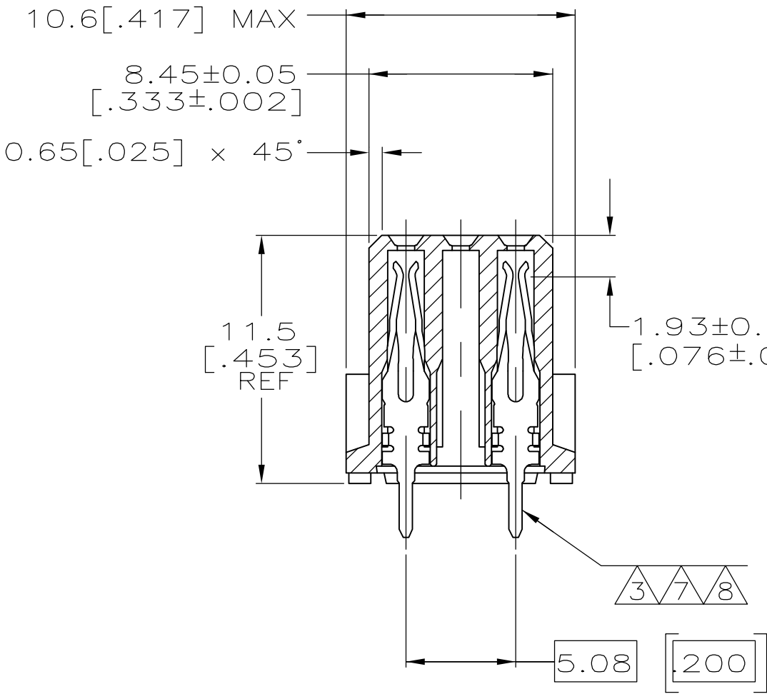
SECTION X-X
