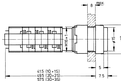
Mounting hole
