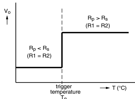
Fig. 2 Typical switch characteristic
