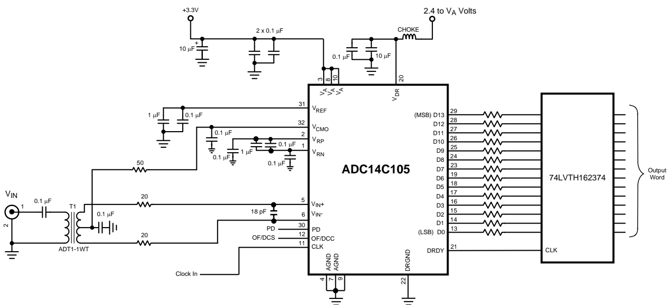
Figure 36. Application Circuit
