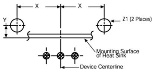
Mounting Details
