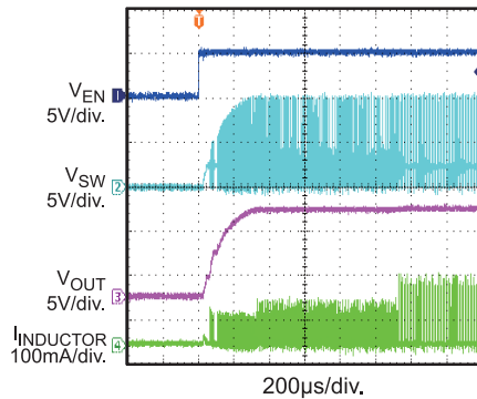
V_{EN} Power On
