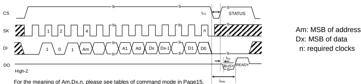
Figure 36. Write Cycle
