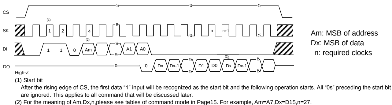
Figure 35. Read Cycle
