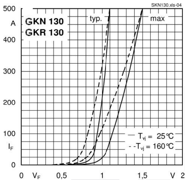
Fig 1: Forward Characteristics
