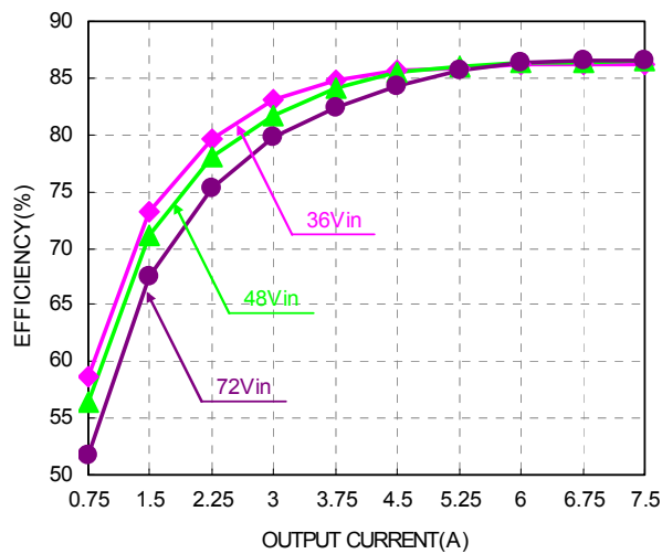
Figure 1: Efficiency vs. load current for minimum, nominal, and maximum input voltage.
