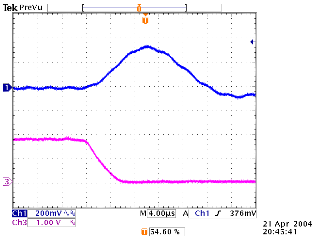
Figure 25: Typical transient response to step load change at 2.5A/µs from 100% to 50% of I_o , max at 3.3Vin, 1.8Vout (Cout = 1µF ceramic, 10µF tantalum)
