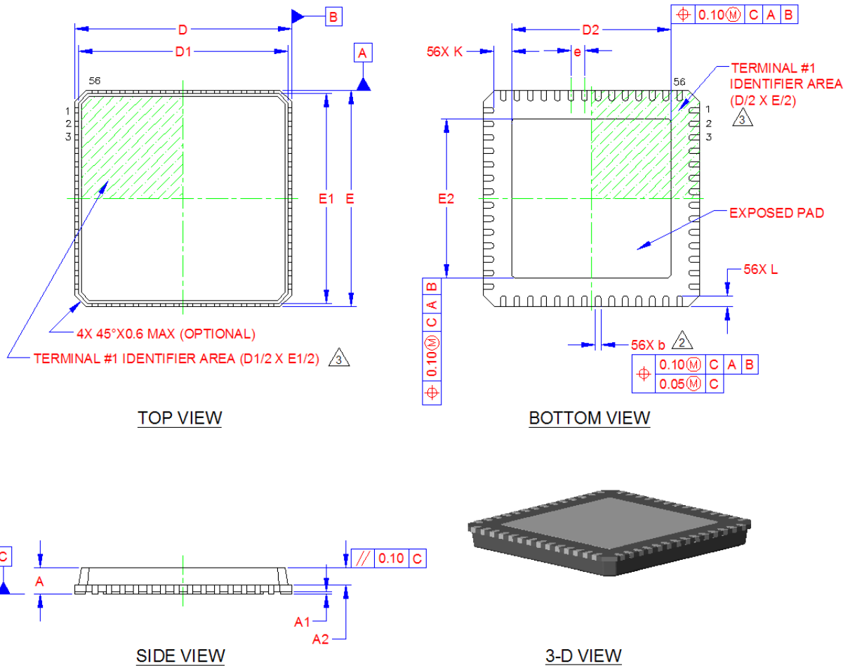
Figure 2 56-QFN Package
