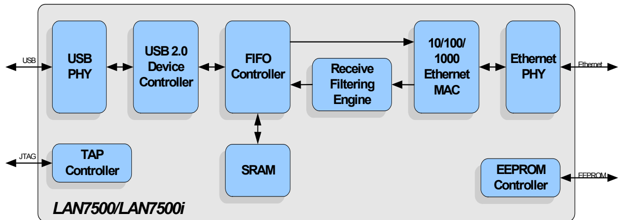
Figure 1 LAN7500/LAN7500i System Diagram
