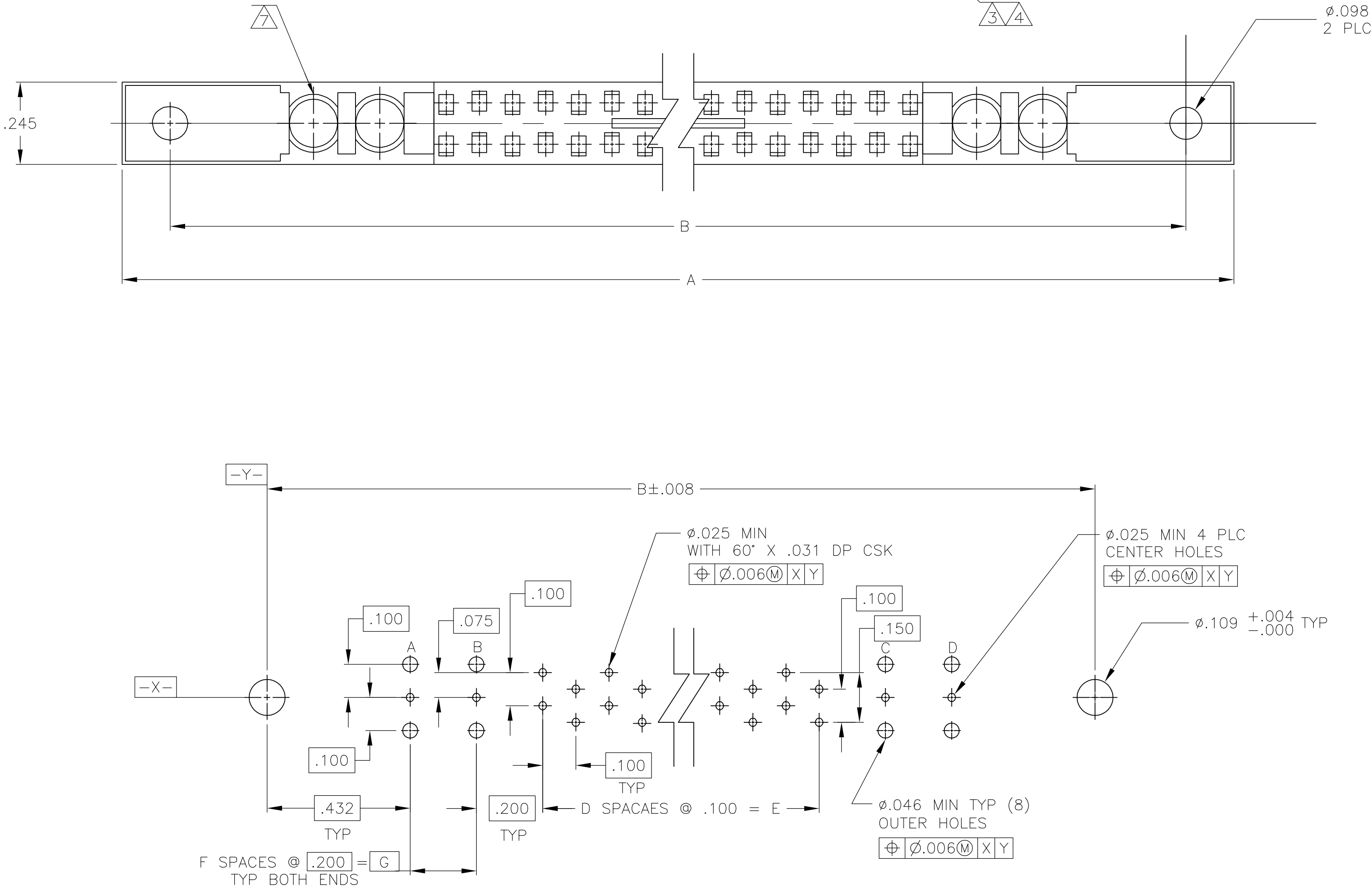
RECOMMENDED BOARD LAYOUT FOR CONNECTORS WITH VERTICAL COAX PC BOARD CONTACTS
