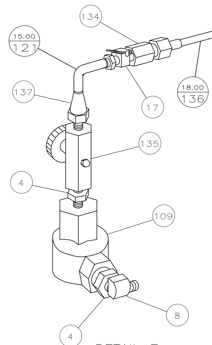
DETAIL E FOR -7 ONLY
