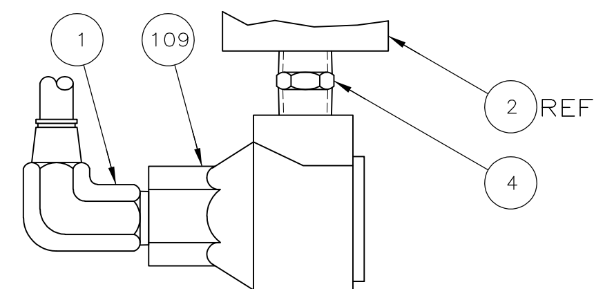
VIEW A-A FOR -1,-3,-4 &-6
