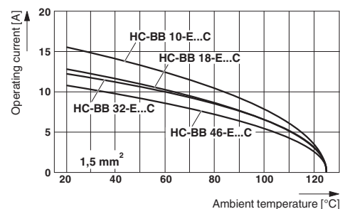
Derating diagram: Conductor cross section 1.5 mm²
