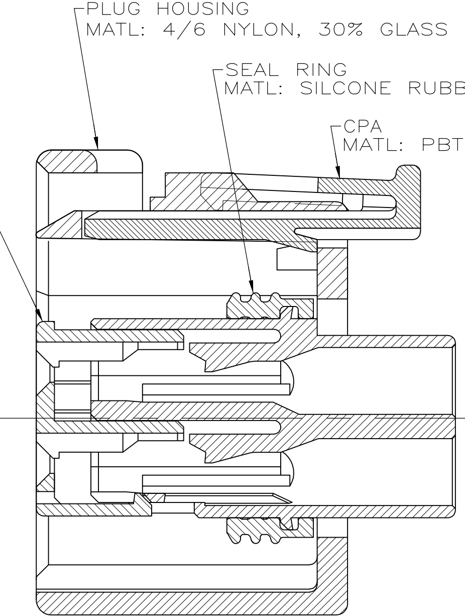
SECTION Z-Z SCALE 4:1
