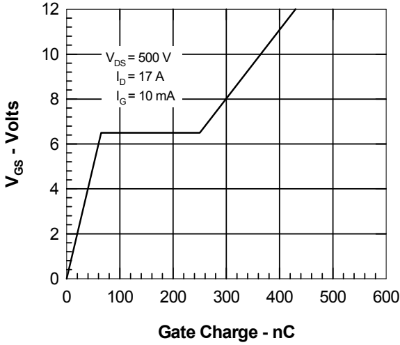
Figure 7. Gate Charge
