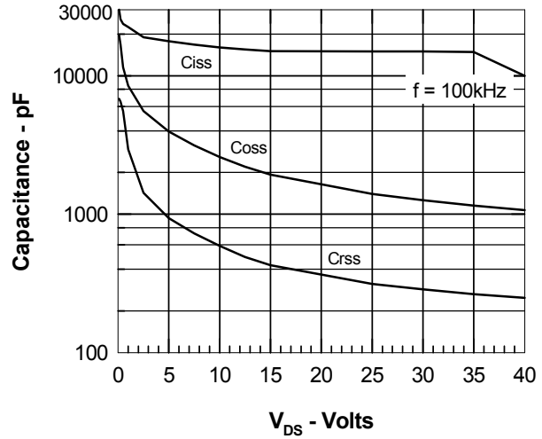
Figure 8. Capacitance Curves
