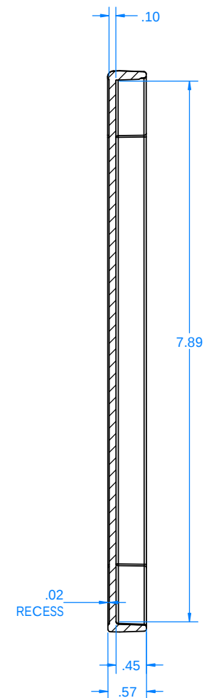
SECTION E-E SCALE 1 : 1
