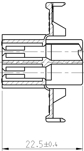
Section A-A SECTION
