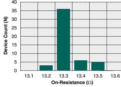
Typical On-Resistance Distribution (N=50, I F =5mA, I L =150mA)
