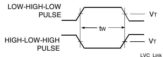
Pulse Width
