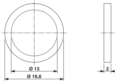
Dimensional drawing
