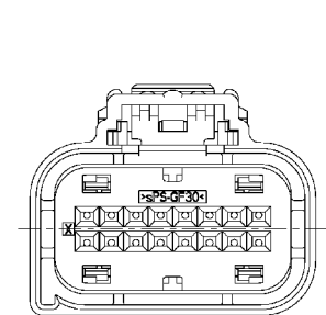
Keying Option "D" (Housing Color : Green)
