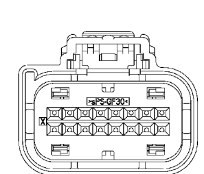
Keying Option "B" (Housing Color: Grey)
