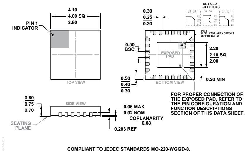
COMPLIANT TO JEDEC STANDARDS MO-220-WGGD-8. Figure 43. 24-Lead Lead Frame Chip Scale Package [LFCSP] 4 mm × 4 mm Body and 0.75 mm Package Height (CP-24-10) Dimensions shown in millimeters
