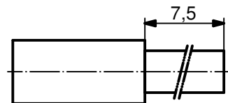
STRIPPING DIMENSIONS
