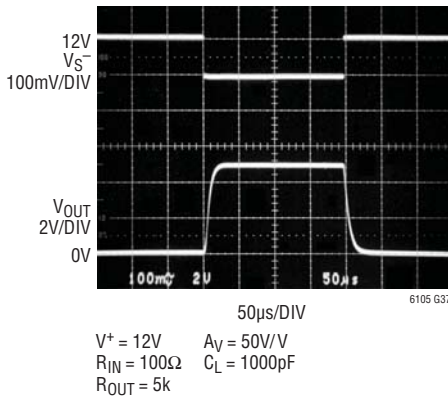
Step Response V_{SENSE} = 0V to 100mV , C_L = 1000pF , V_{S^+} = 12V
