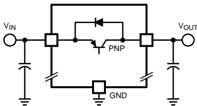
Figure 23. Normal Operation
