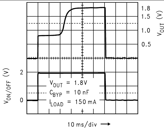
Figure 35. Turnon Time
