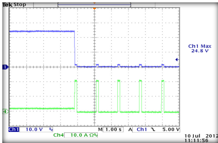
24V OUT, 264VAC
