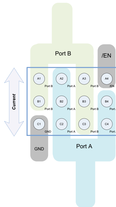
Fig. 21 - Proposed Layout
