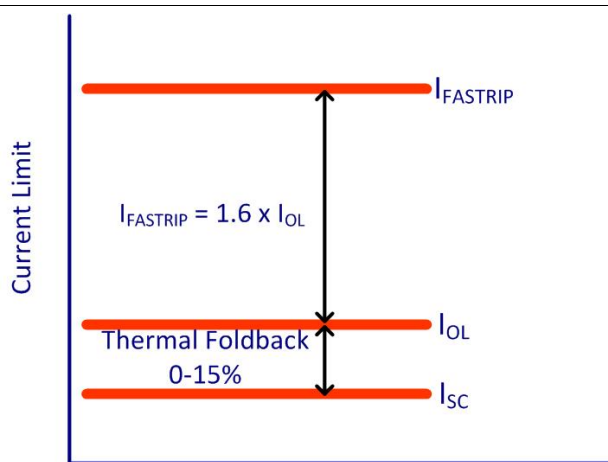
Figure 36. Fast-Trip Current
