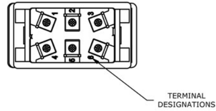
Double Pole with actuator
