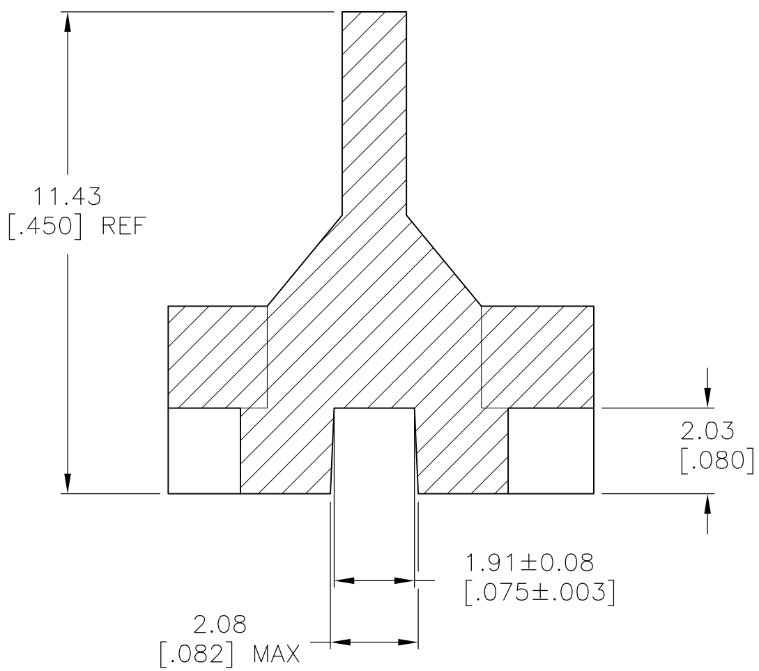
SECTION X-X SCALE 8:1
